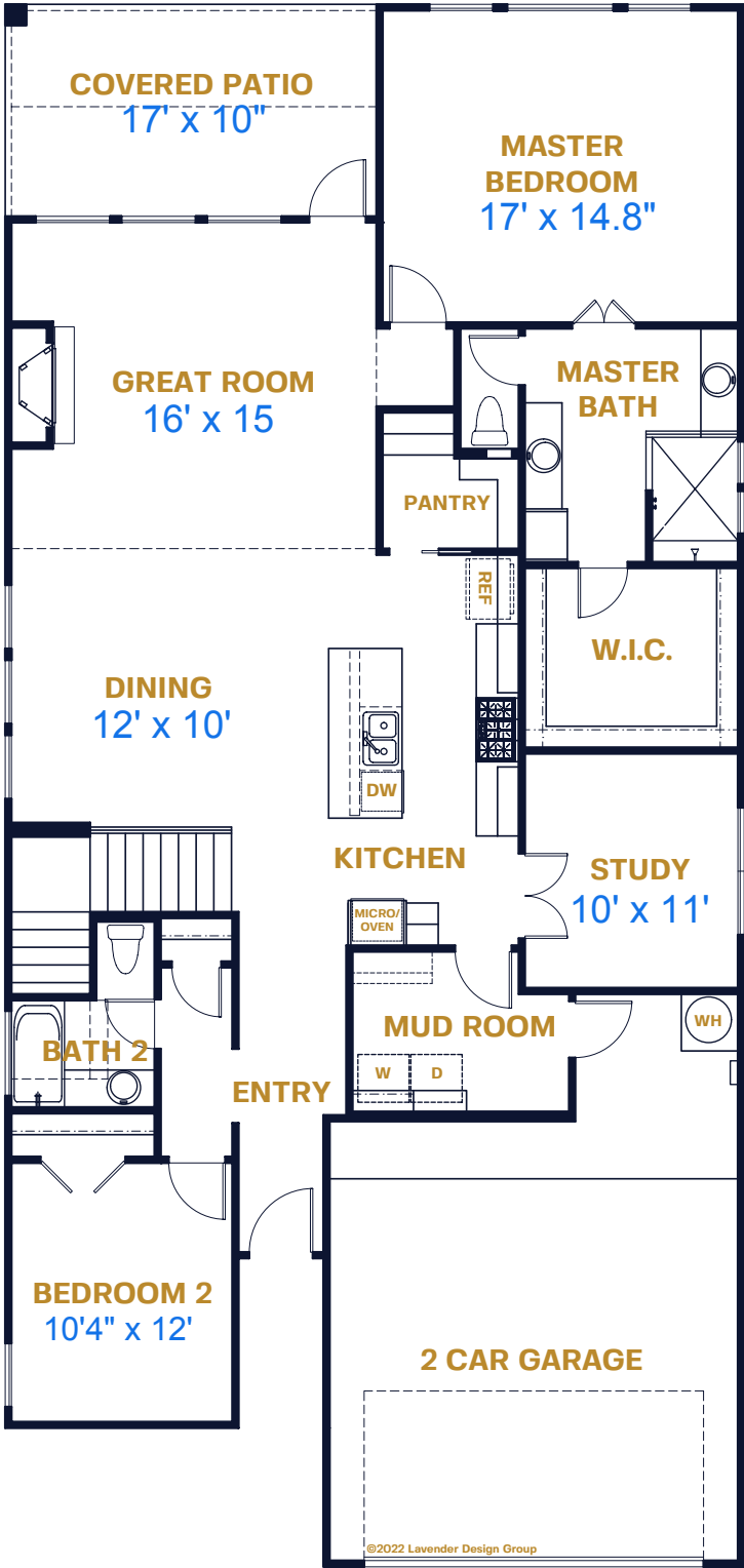
FIRST FLOOR
